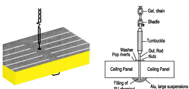
Polyurethane ceiling panel big suspension joint
