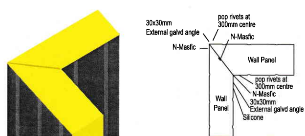
Polyurethane wall to wall panel corner joint detail
