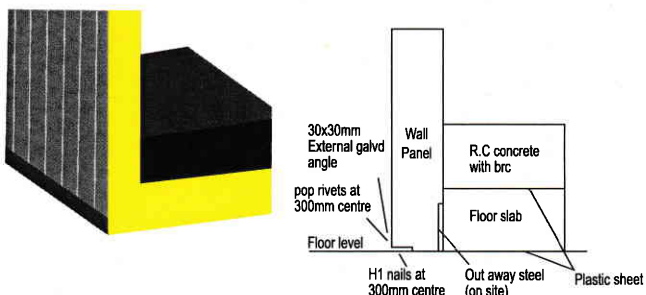
Polyurethane finishing floor sectional
