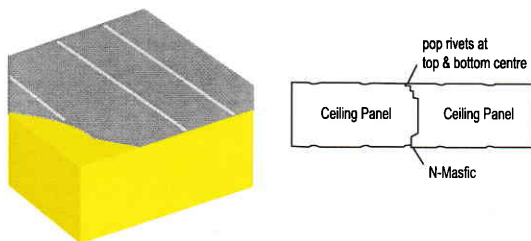
Polyurethane ceiling to ceiling panel joint detail
