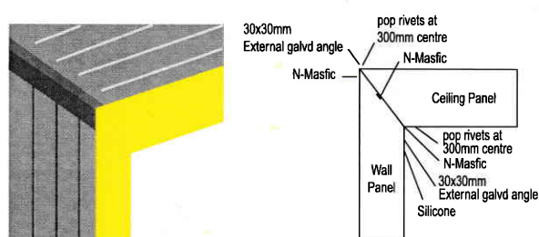
Polyurethane wall to ceiling panel corner joint detail
