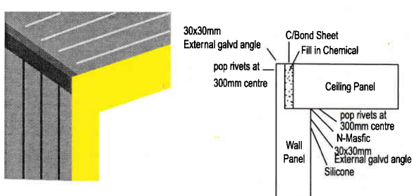
Polyurethane wall to ceiling panel corner joint detail
