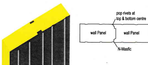
Polyurethane wall to wall panel joint detail
