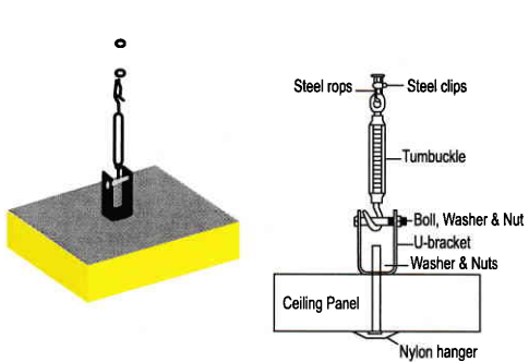
Polyurethane ceiling panel nylon hanger joint
